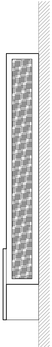
WS2647 11" W x 4" PROJ 30" OVERALL HEIGHT MACHINED ALUMINUM TEXTURED ACRYLIC DIFFUSER WITH SANDBLASTED FINISH OUTSIDE
