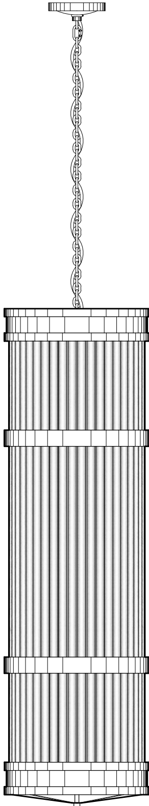
P2265 18" DIA x 61" H STAINLESS STEEL METALWORK 1" DIAMETER CLEAR GLASS TUBES
