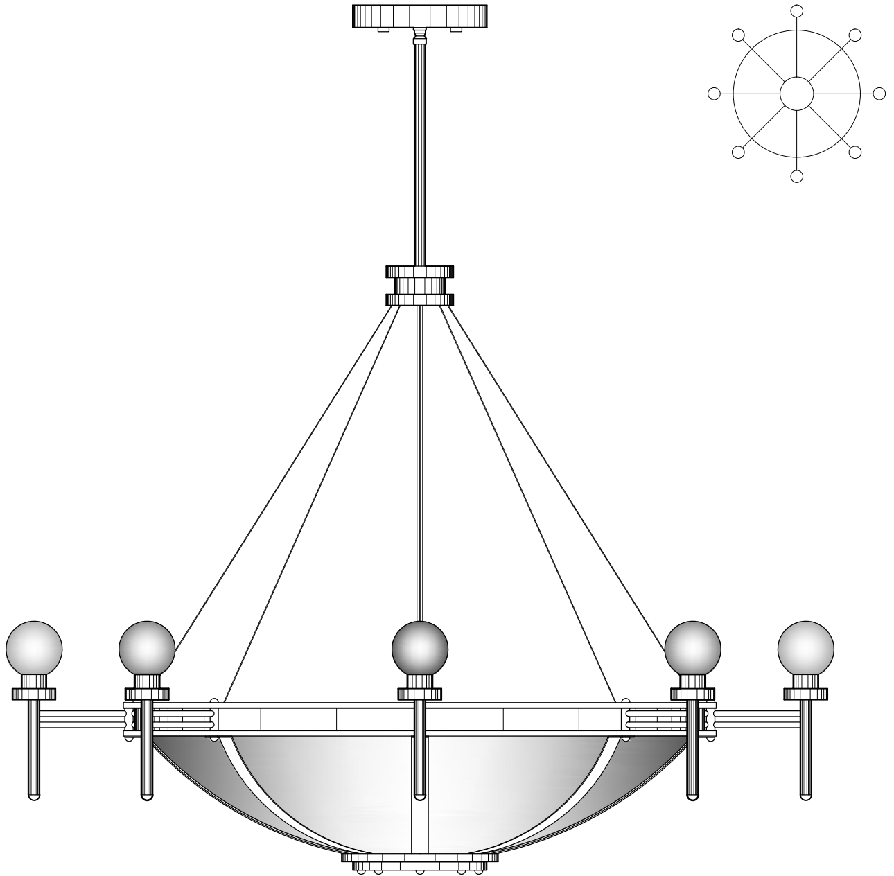
P1445 49" DIAMETER BRONZE METALWORK TRANSLUCENT WHITE ACRYLIC BOWL
