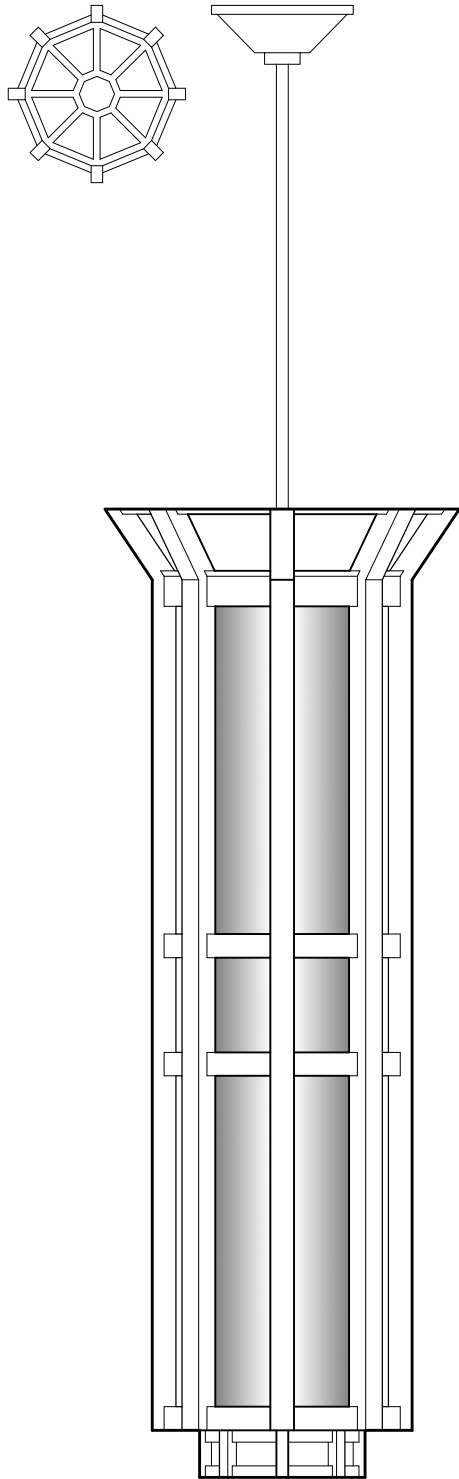
P1259 12" DIA x 82" H ALUMINUM METALWORK TRANSLUCENT WHITE ACRYLIC PANELS
